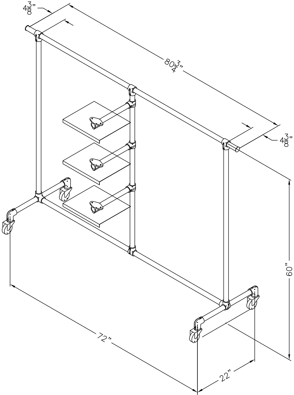
ROLLING RACK 72" L x 60" H x 22" W
