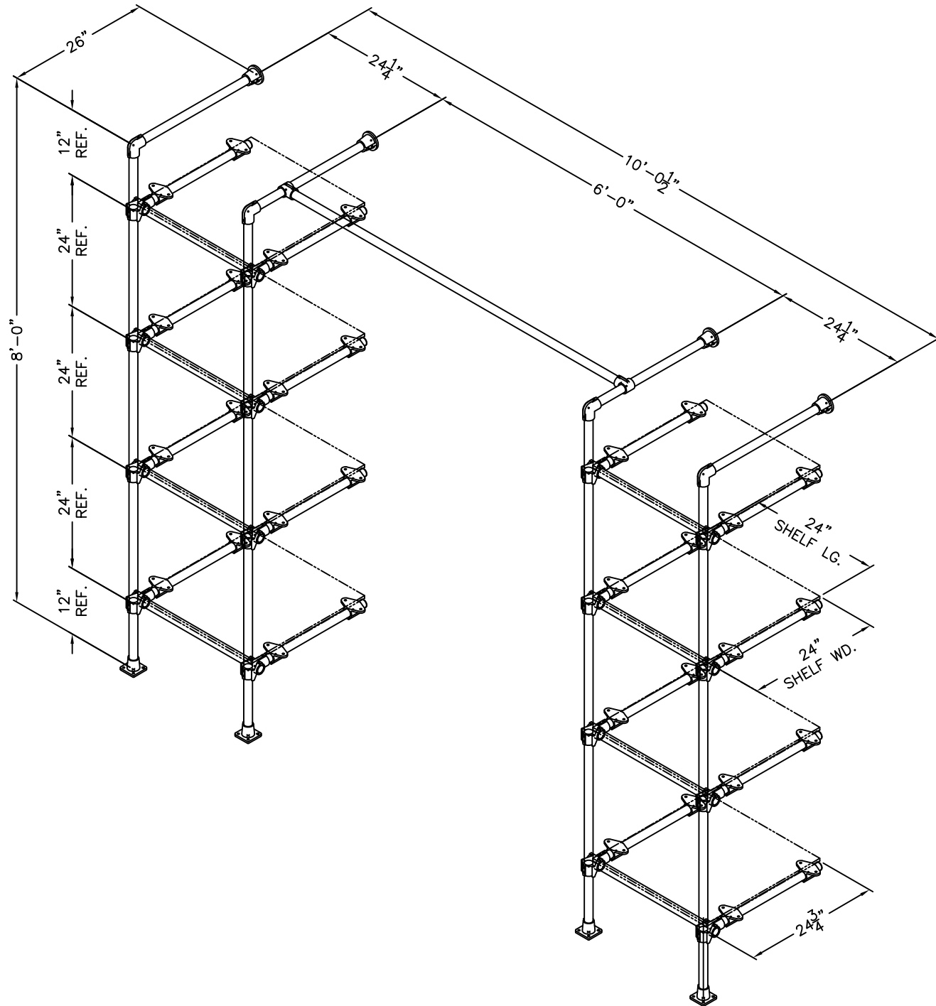
WALL RACK "F" 10'-0" x 8'-0" w/ 24" DP. SHELVES
