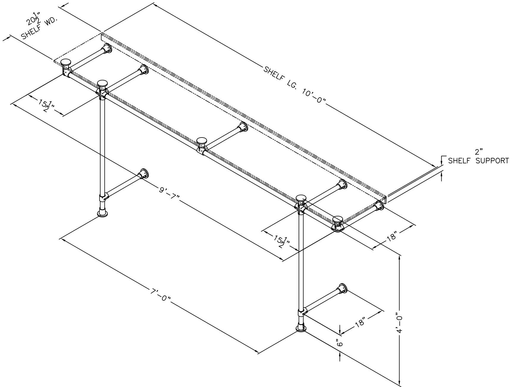
WALL RACK "H" 10'-0" x 18" w/ 22 1/2" SHELF
